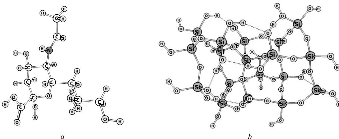
Fig. 2. Models: a – N -acetylneuraminic acid, b – silica cluster
