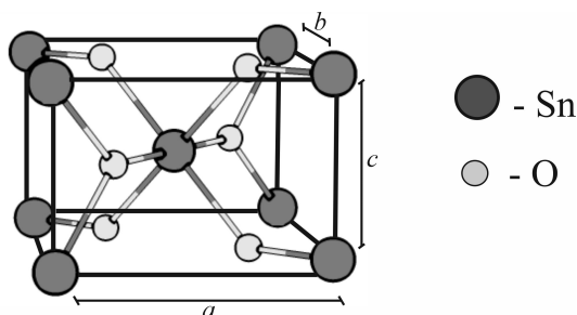
Fig. 1. The structure of the SnO 2 unit cell [3]
